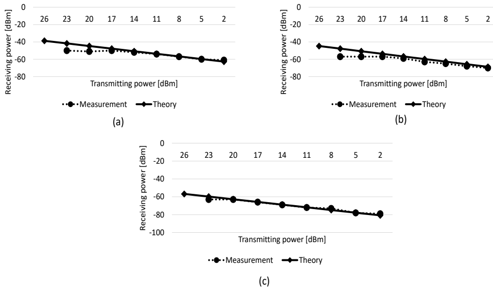
Fig. 6. Comparison between theory and measured receiving power at channel 36 – 5.18GHz (a) 10m, (b) 20m and (c) 80m
