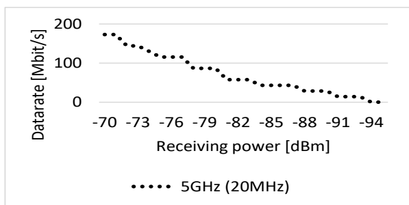
Fig. 4. – Sensibility of the WLE600VX WLAN module, IEEE802.11n, 20MHz [16]
