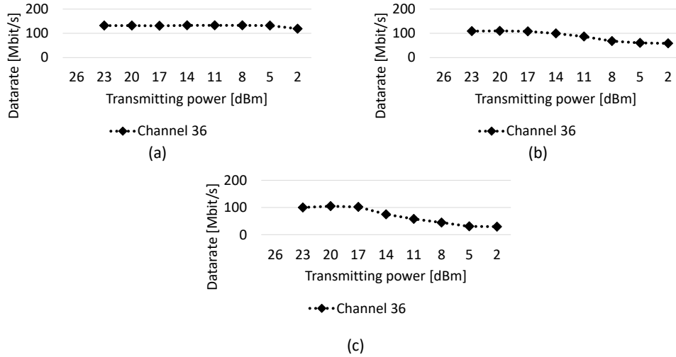
Fig. 8. Measured TCP bitrate depending on the transmission power at channel 36 – 5.18GHz (a) 10m, (b) 20m and (c) 80m
