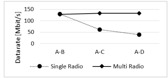
Fig. 12. TCP throughput depending of the number hop
