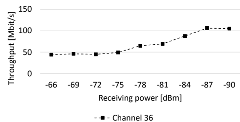
Fig. 10. Throughput depending of the receiving power of the disturber
