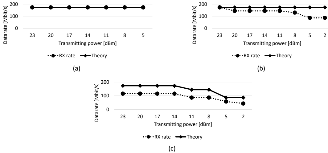
Fig. 7. Comparison between the measured RX rate and the expected value according to the measured receiving power at channel 36 – 5.18GHz (a) 10m, (b) 20m and (c) 80m
